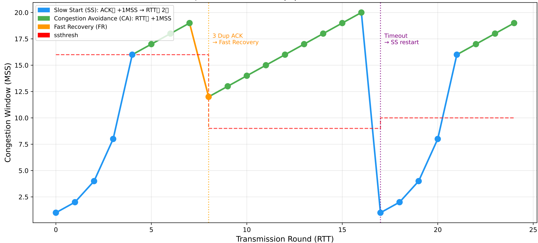
TCP Reno: cwnd Evolution (RTT=8: 3 Dup ACK → Fast Recovery | RTT=17: Timeout → Slow Start)
